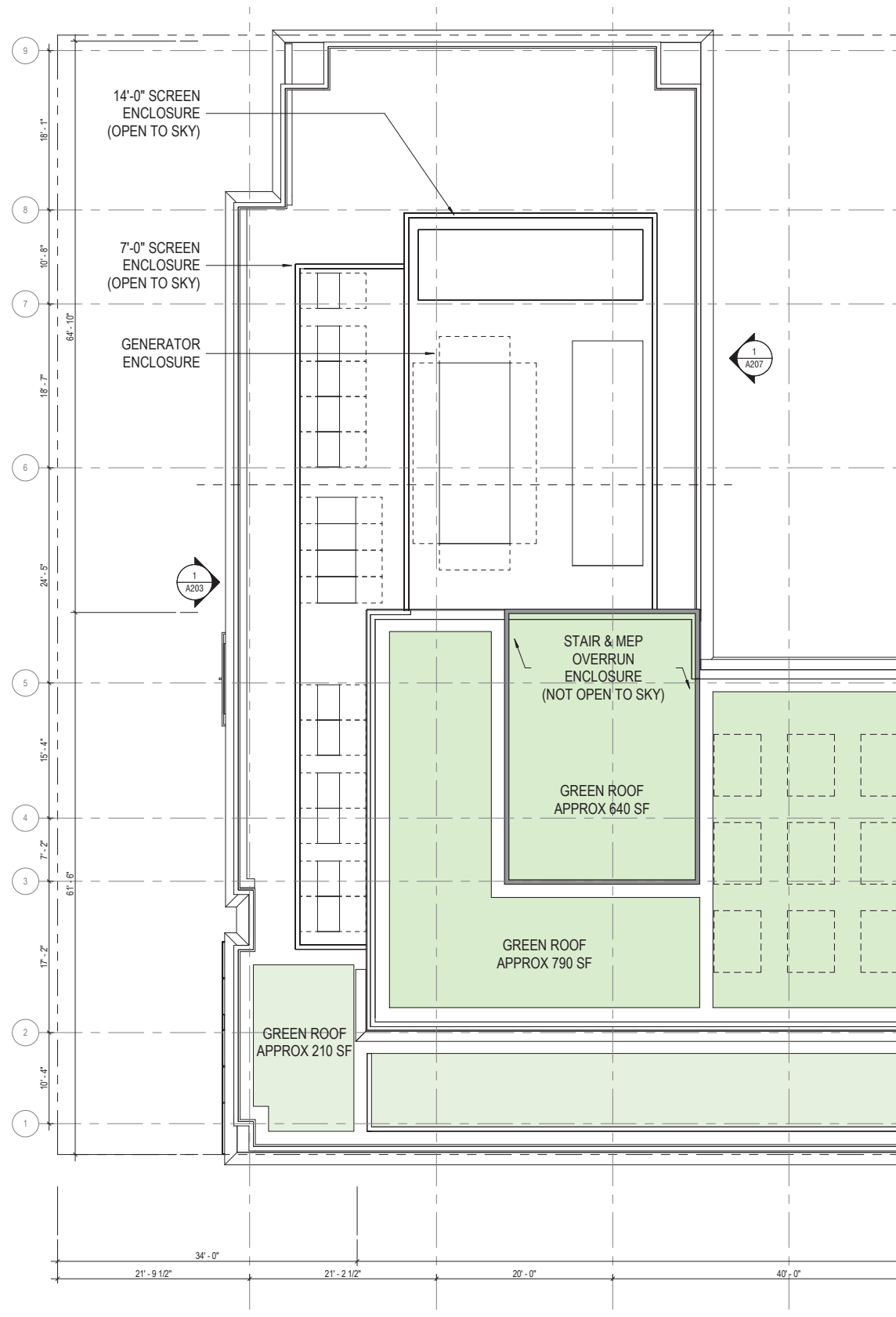
Roof Plan Detail
