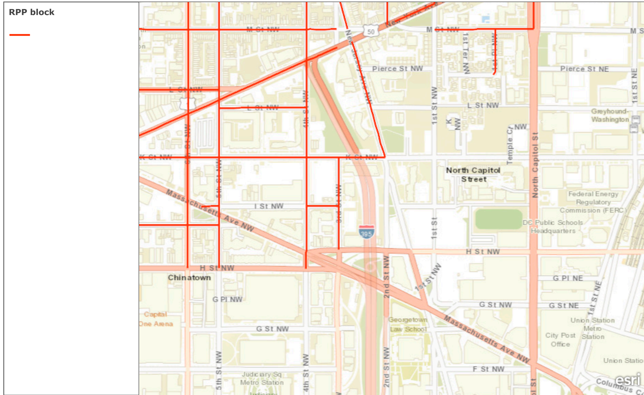
Map showing designated RPP blocks within the District
