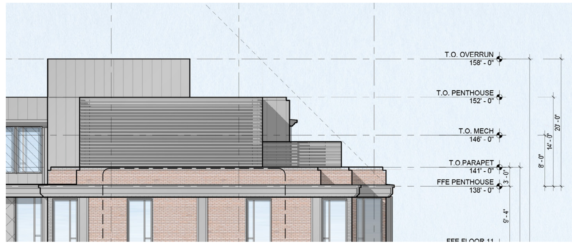
North Elevation Detail
