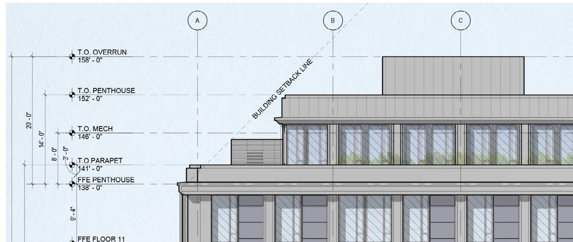
South Elevation Detail
